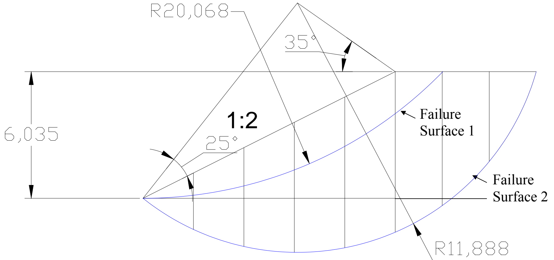
Fig.3.41: Slope Stability Analysis for Embankment along Road No. 10.
